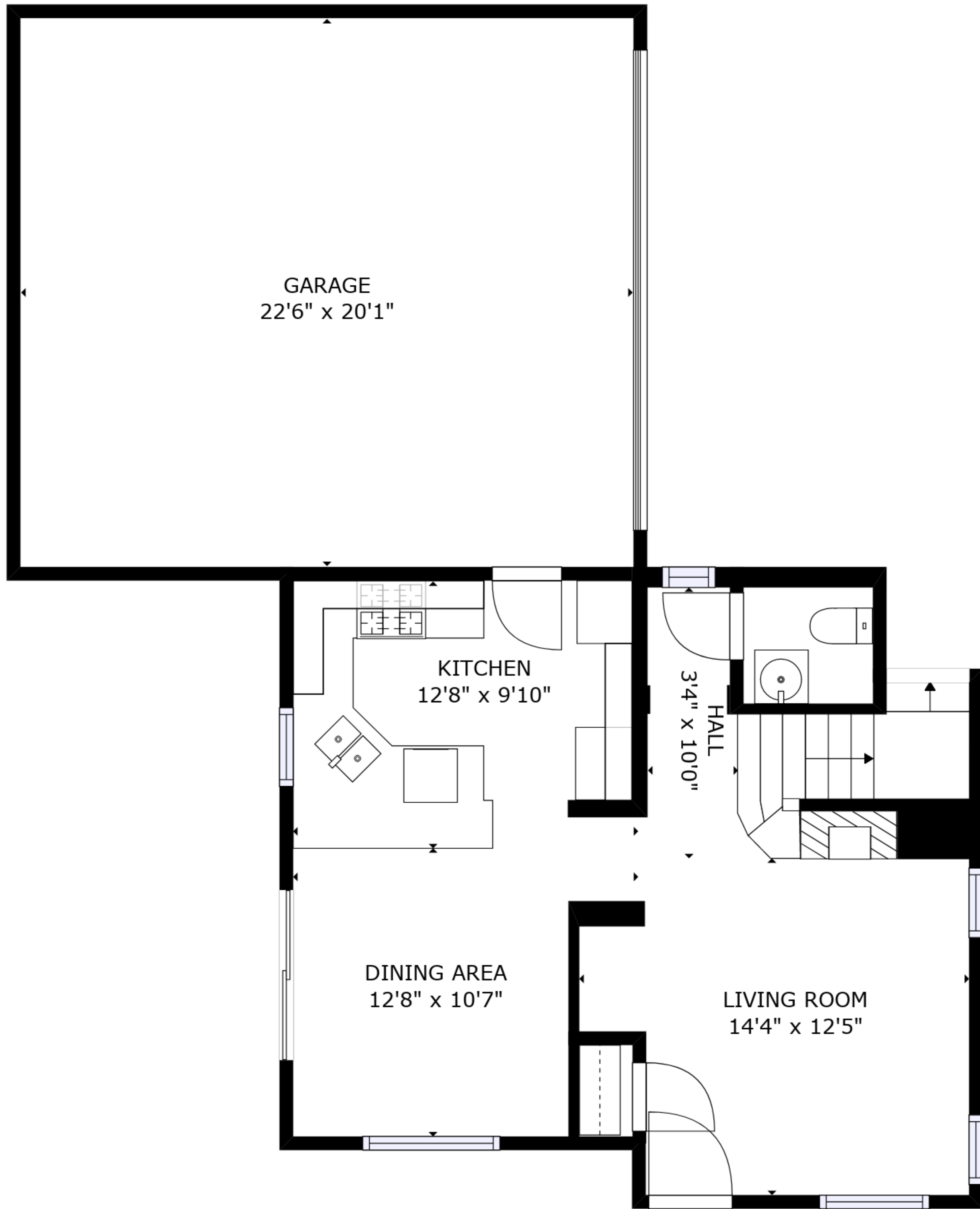
FLOOR 1
