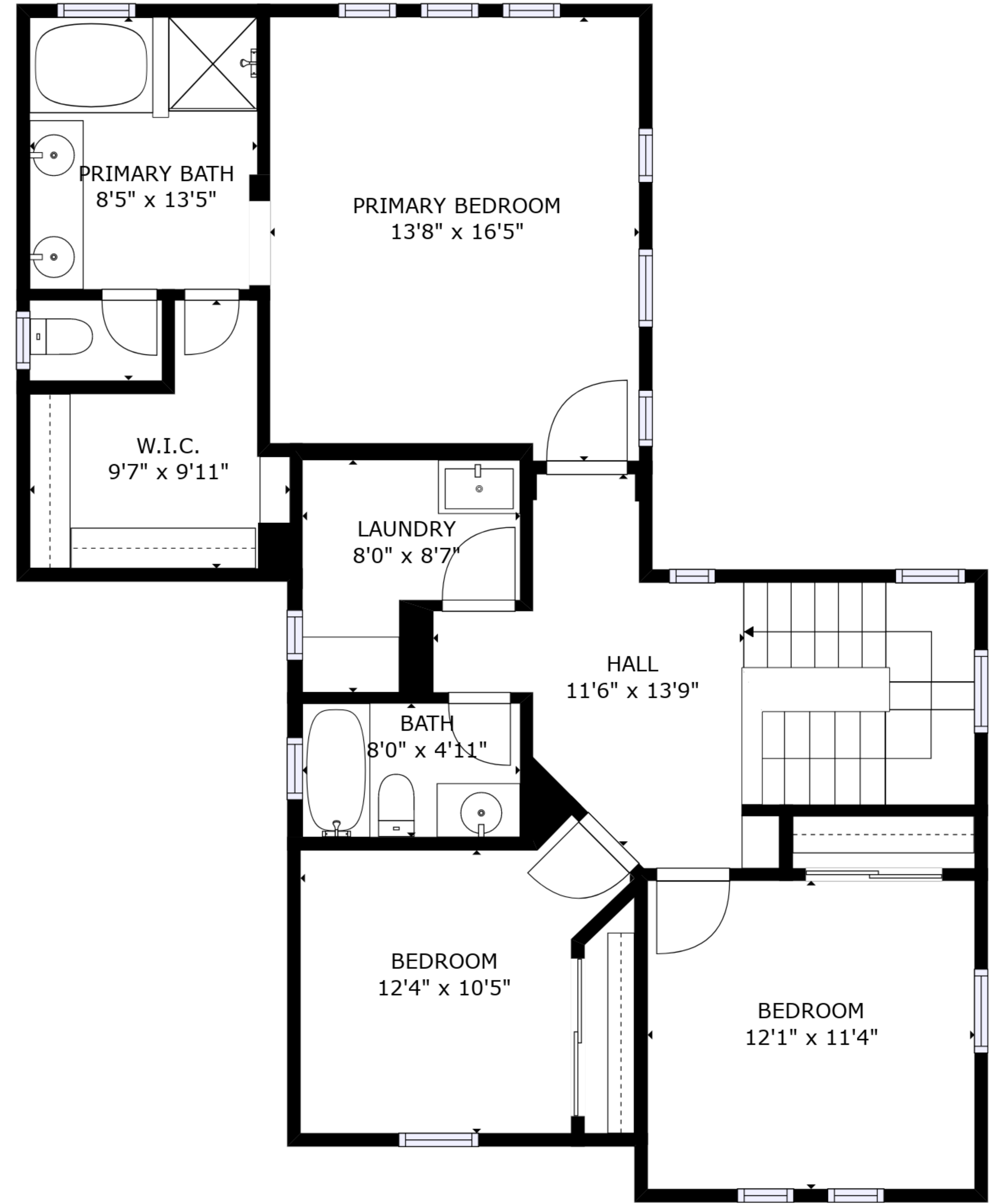
FLOOR 2
