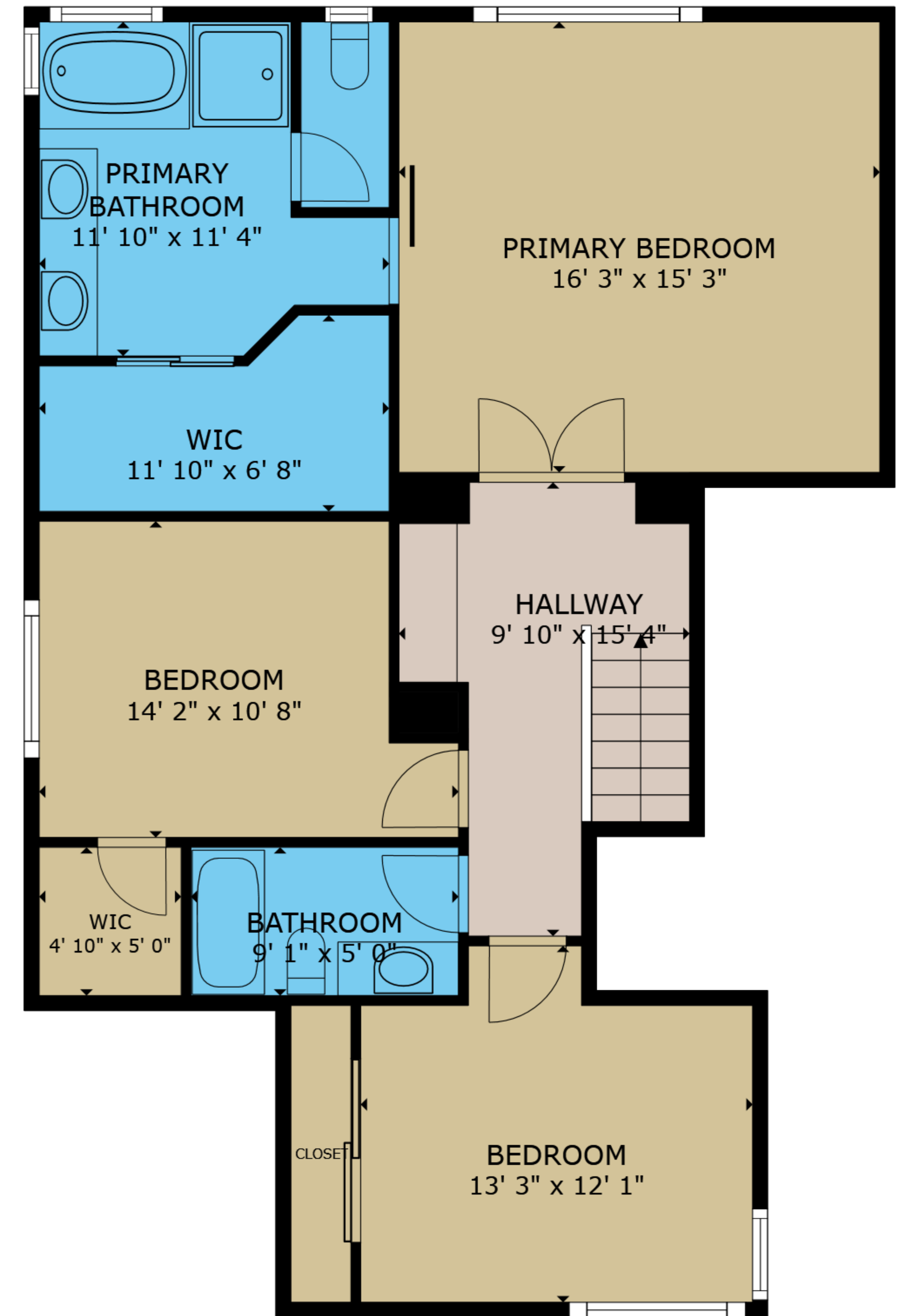
FLOOR 2
