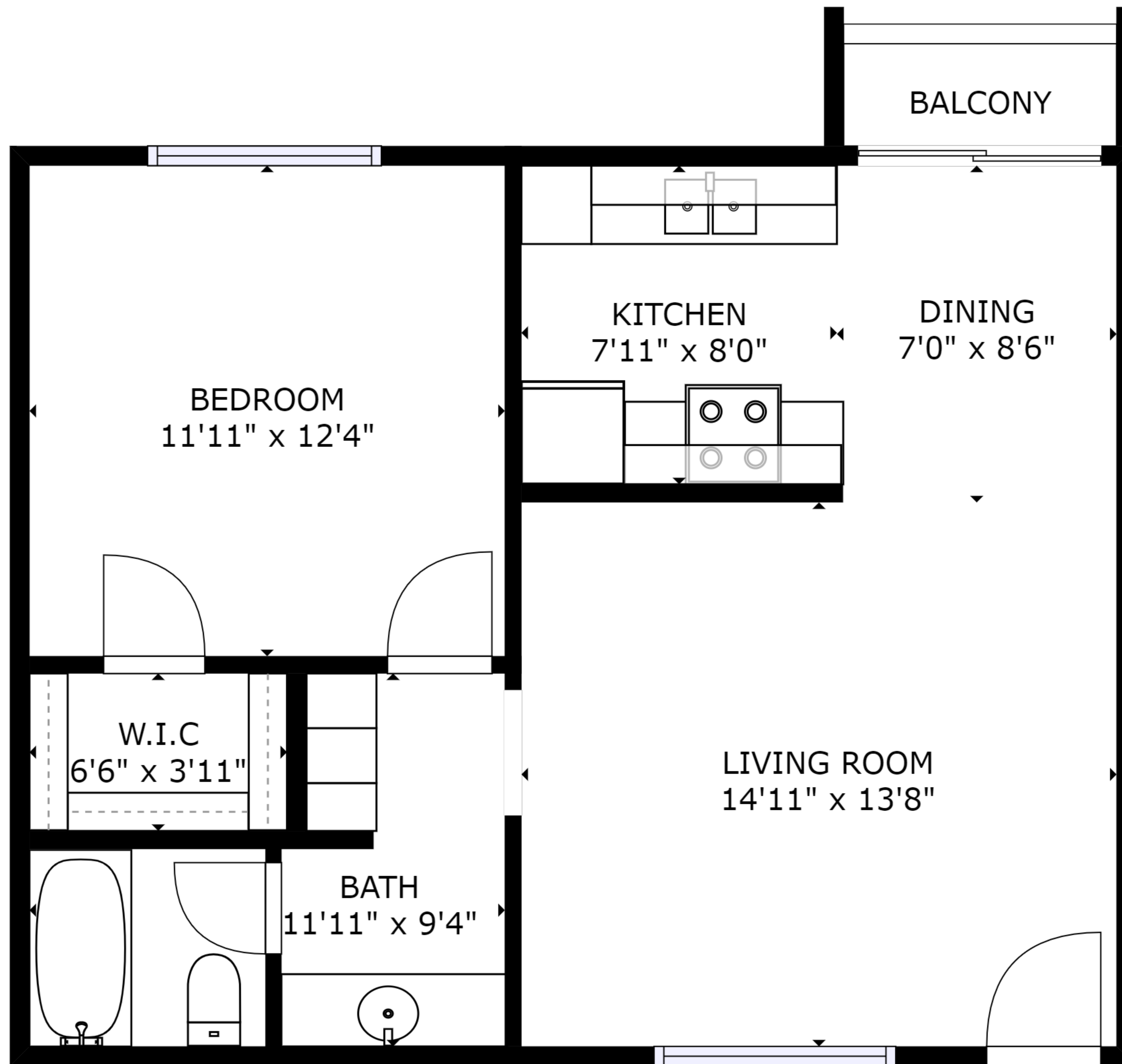
FLOOR 1
