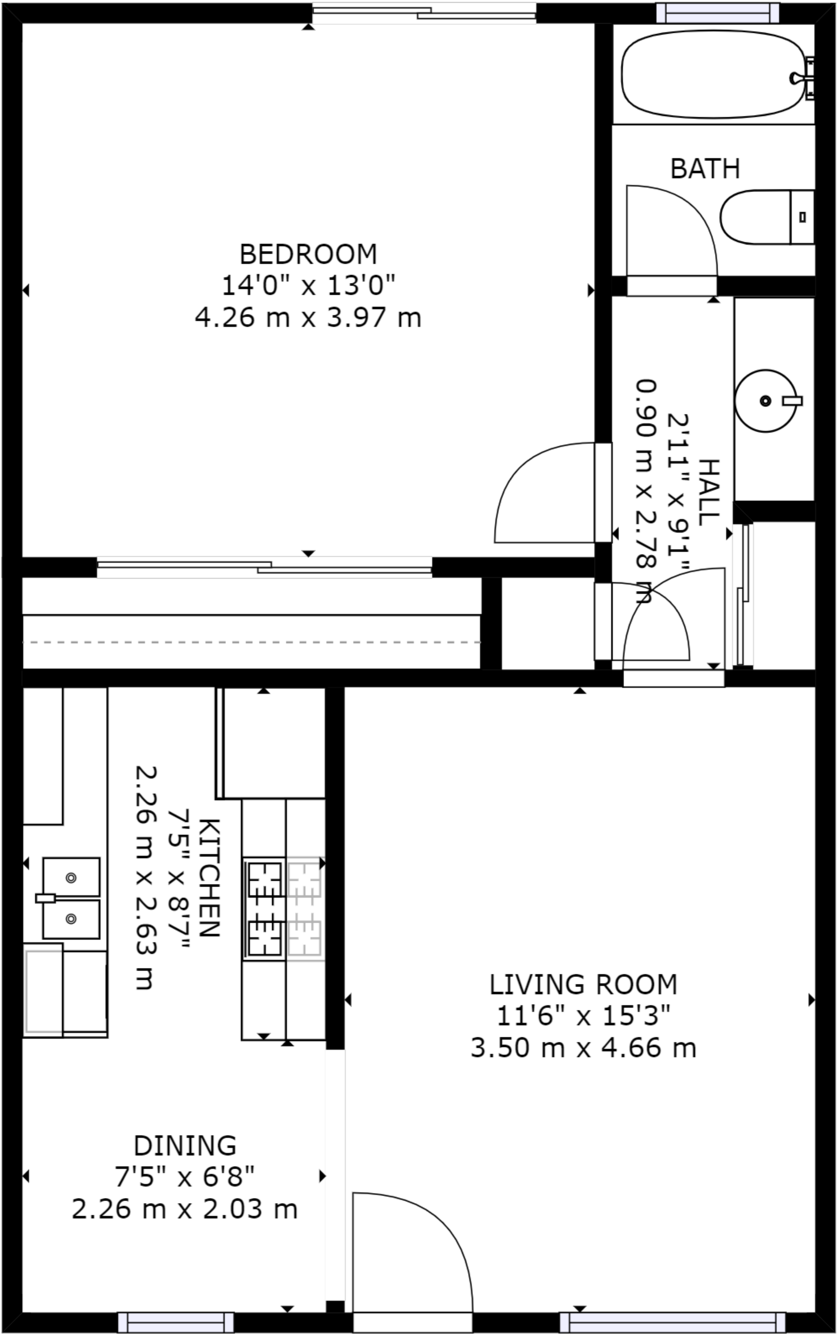
FLOOR 1
